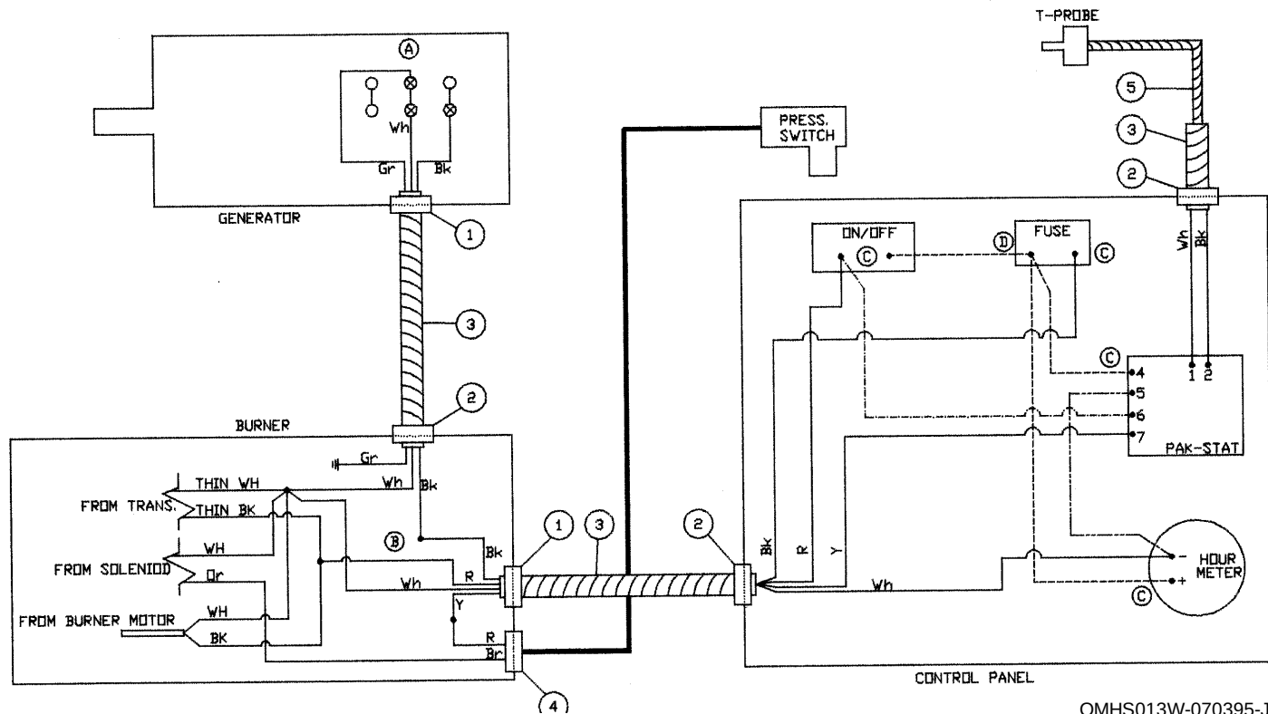
WIRING DIAGRAM FOR HS-2204-CMH1 & HS-2505/3005-CMV1
